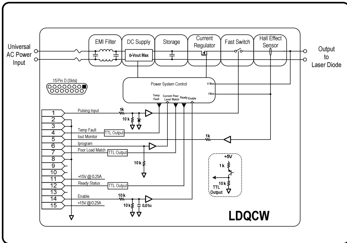
Figure 1 - LDQCW Block Diagram
