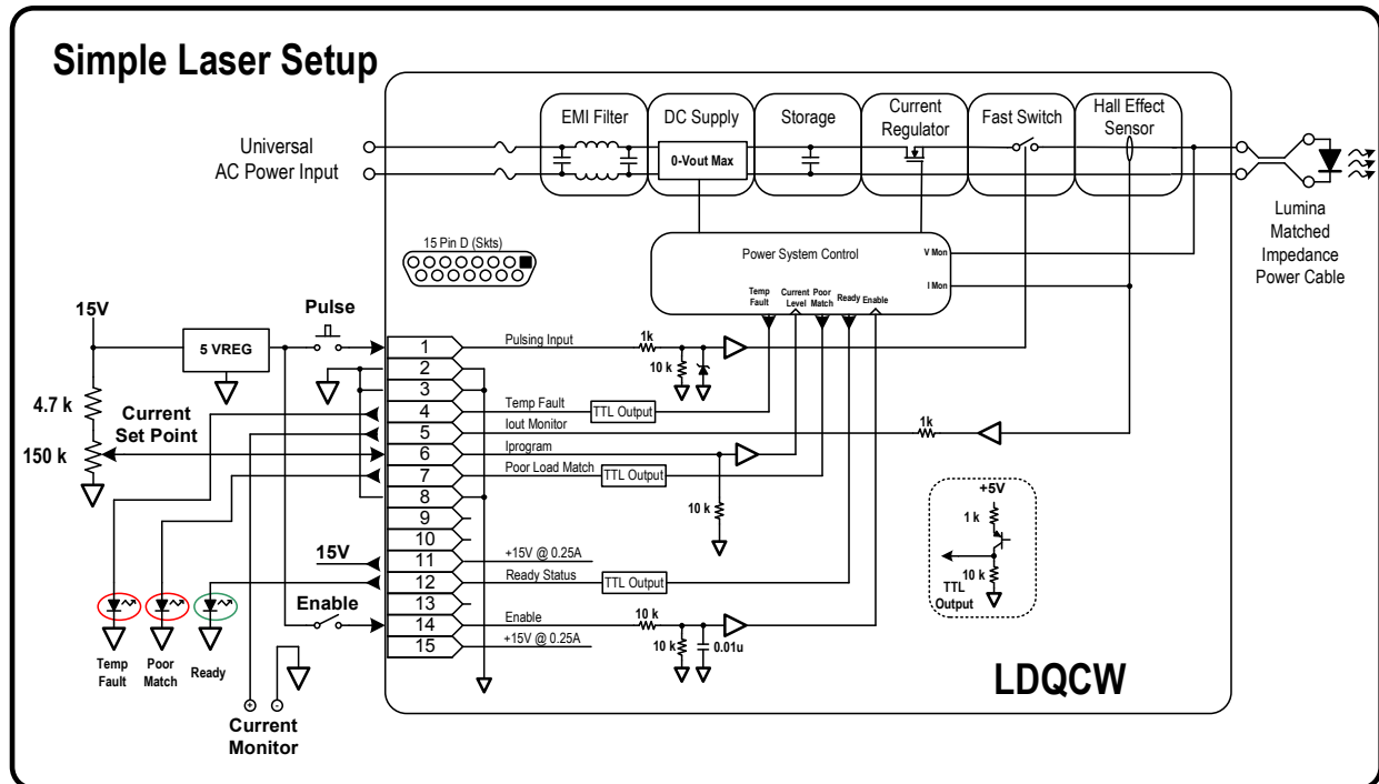
Figure 4 - Simple Laser Setup
