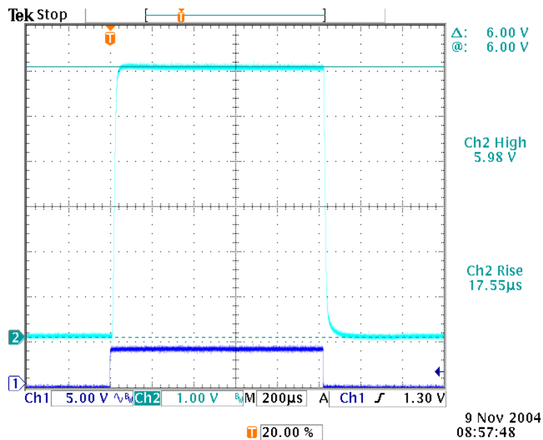
Figure 3 -Typical Rise/Fall Time
