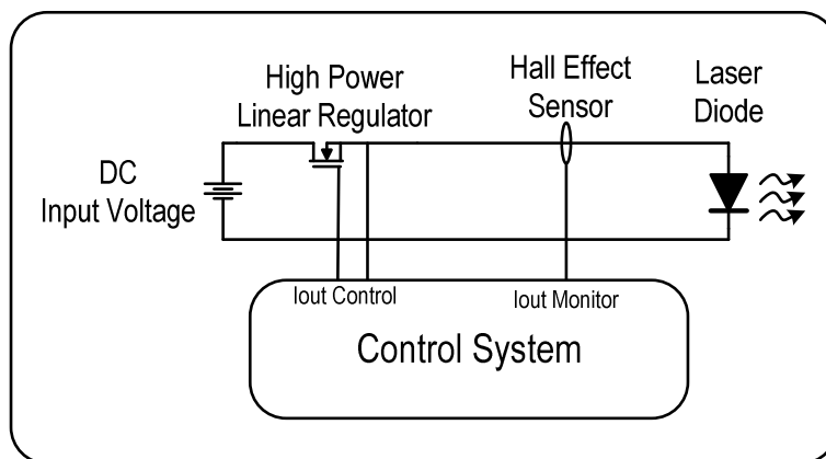
Figure 2 - Simplified LDQCW Block Diagram
